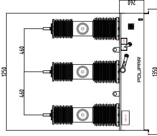
24 kV AUTO RECLOSER MAIN BODY
